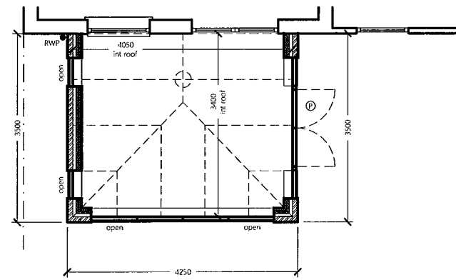
PROPOSED PLAN VIEW
