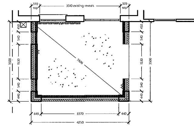
PROPOSED BASEWORK LAYOUT
